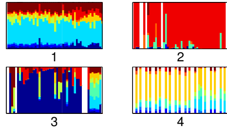
(b) Time-evolving Mixed-Memberships
